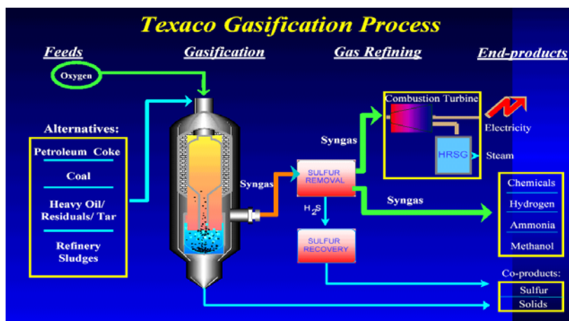
Figure 5 Downdraft entrained-flow Texaco gasifier. Gasification process is versatile in the feedstock choice as well as the end-product spectrum following from further processing of syngas.
