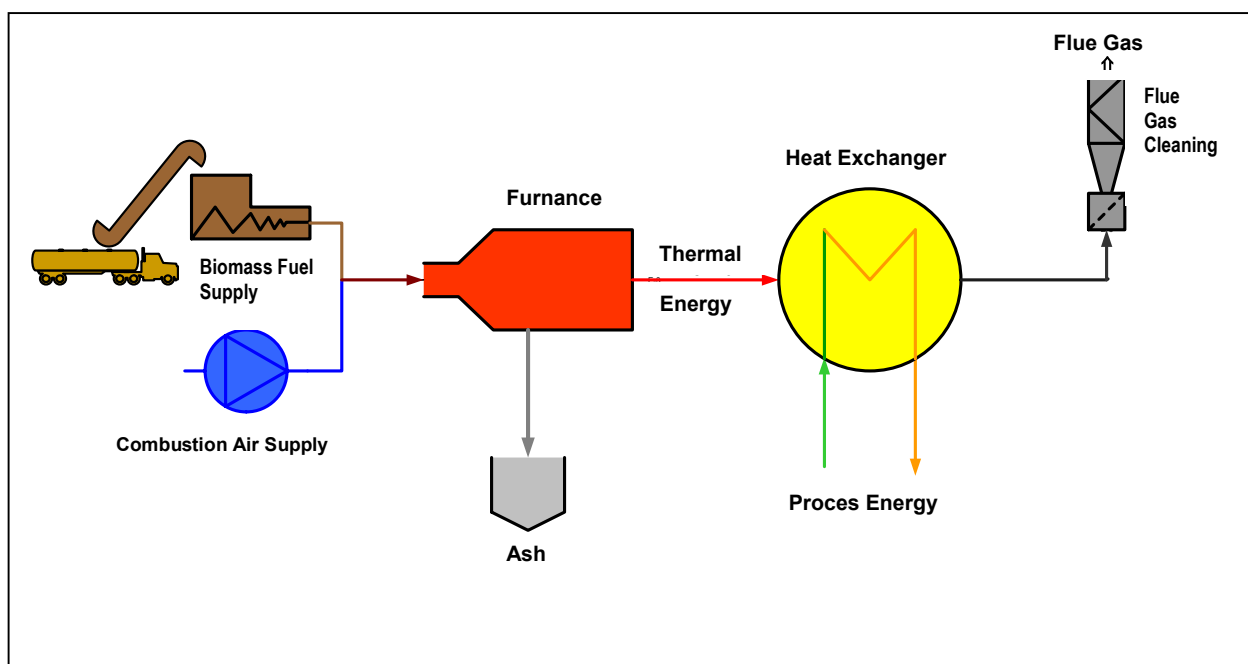
Figure 2 Principal scheme of direct combustion system
