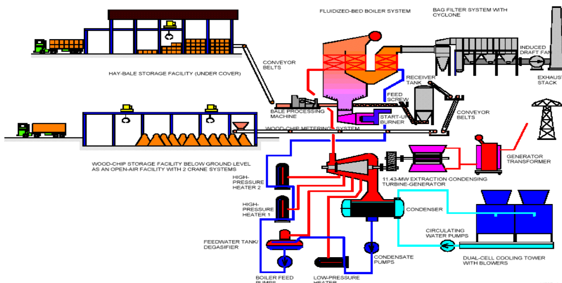
Figure 3 Typical Scheme of Biomass Fired Power Generation Plant (Courtesy of SIEMENS)
