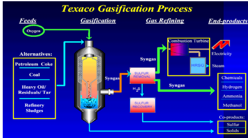
Figure 5 Downdraft entrained-flow Texaco gasifier.
