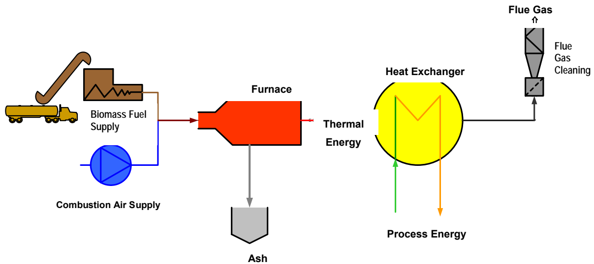
Figure 2 Principal scheme of direct combustion system
